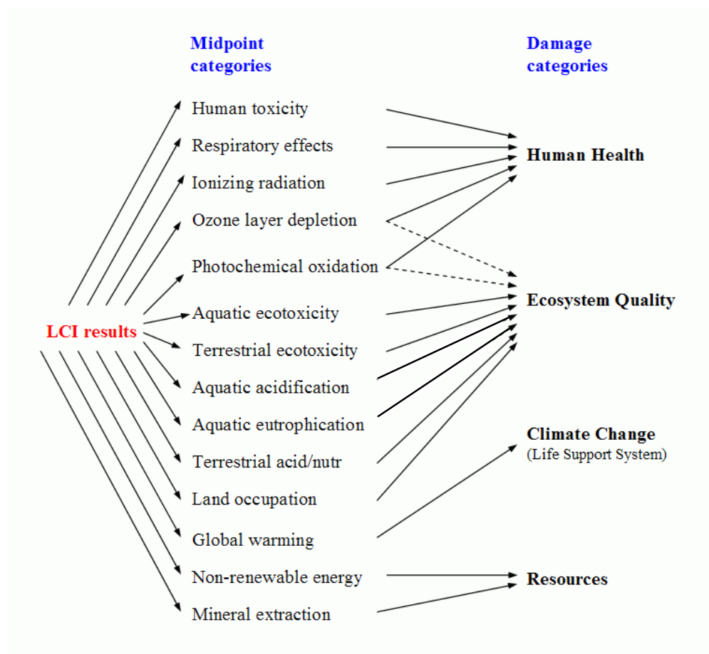
Figure B-1: Overall schematic of IMPACT 2002+ (version 2.15 used by CIRAIG), linking the life cycle inventory results (LCI) and the damage categories, via the midpoint categories.
